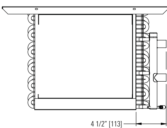
2-PIPE - FRONT VIEW LH SHOWN RH OPPOSITE
