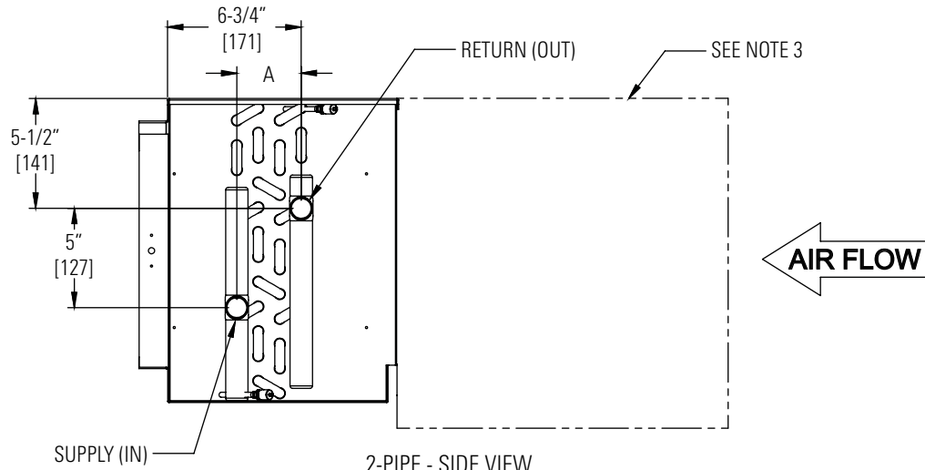
2-PIPE - SIDE VIEW LH SHOWN RH OPPOSITE
