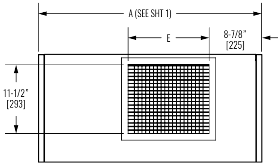
EXTENDED FRONT PANEL GRILLED SUPPLY
