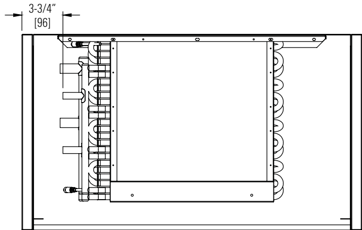
4-PIPE - BACK VIEW LH SHOWN RH OPPOSITE
