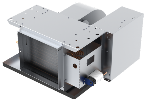
MODEL THHC Horizontal Free Return
