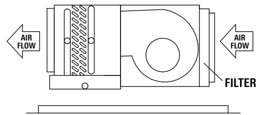
THHP REAR RETURN WITH SOLID ACCESS PANEL
