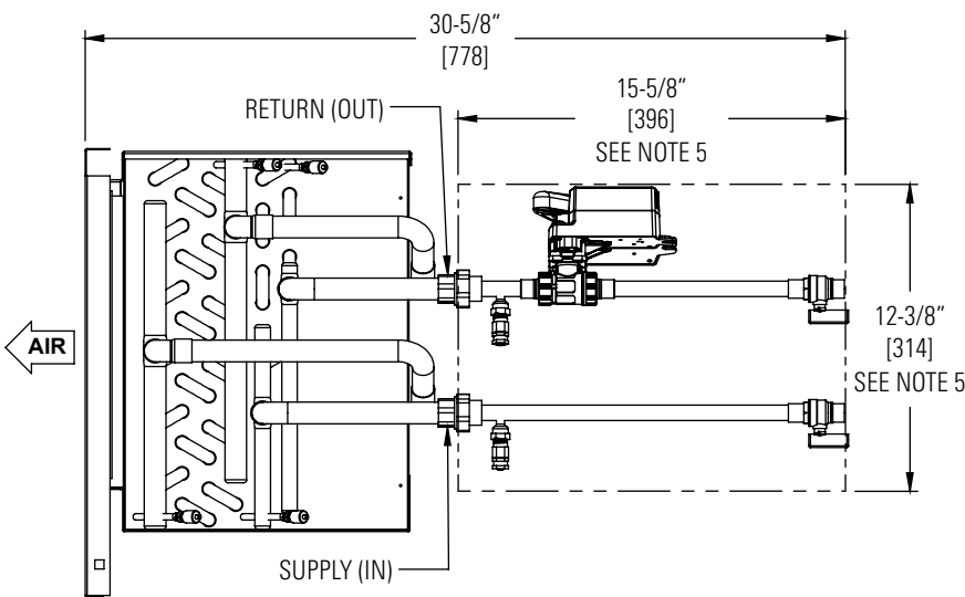
THHE 4 - PIPE WATER COIL (LEFT HAND SHOWN) (RIGHT HAND OPPOSITE)
