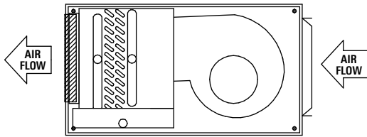
THE DOUBLE DEFLECTION SUPPLY GRILLE AND DUCTED REAR RETURN
