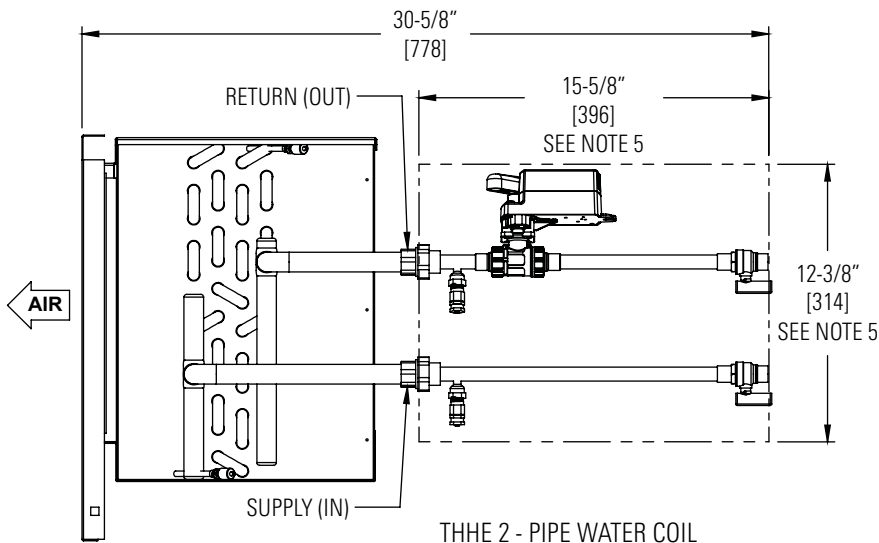
THHE 2 - PIPE WATER COIL (LEFT HAND SHOWN) (RIGHT HAND OPPOSITE)
