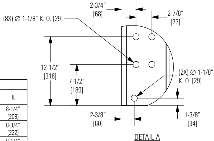
BACK PANEL DUCTED RETURN
