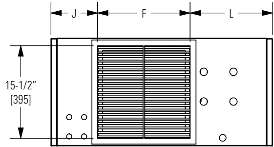
EXTENDED BACK PANEL GRILLED SUPPLY
