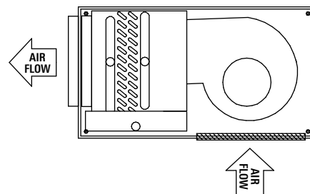
THE DUCTED SUPPLY AND SINGLE DEFLECTION BOTTOM RETURN GRILLE
