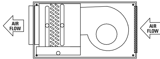
THE DUCTED SUPPLY AND SINGLE DEFLECTION REAR RETURN GRILLE
