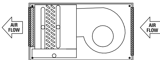
THE DOUBLE DEFLECTION SUPPLY GRILLE AND SINGLE DEFLECTION REAR RETURN GRILLE
