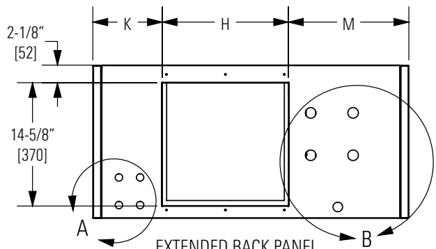
EXTENDED BACK PANEL DUCTED SUPPLY
