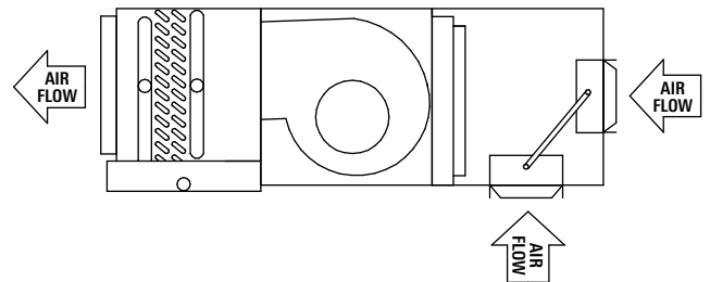
THHP MIXING BOX W/BOTTOM & REAR RETURN
