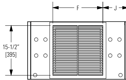
BACK PANEL GRILLED RETURN
