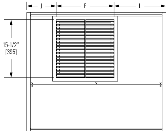
EXTENDED BOTTOM PANEL GRILLED RETURN
