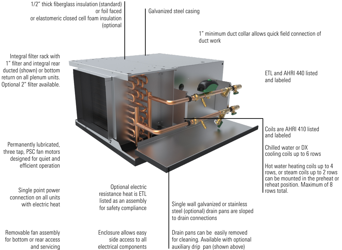
MODEL THHE Horizontal Exposed Cabinet
